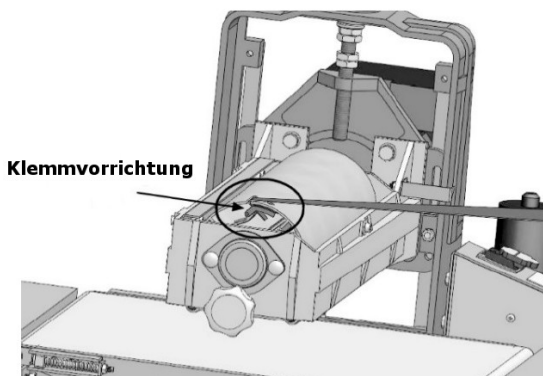
Abb. 22: Klemmvorrichtung links
